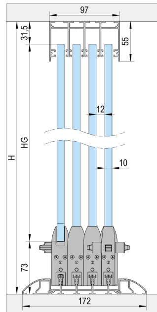
Assembly with recessed track and ramp profiles / 4-panel
