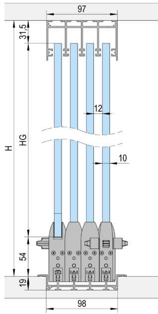
Assembly with recessed track / 4-panel
